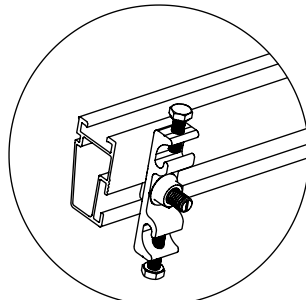
DETALLE "C" NXT-GC Terminal a Tierra
