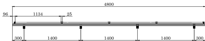
VISTA FRONTAL
